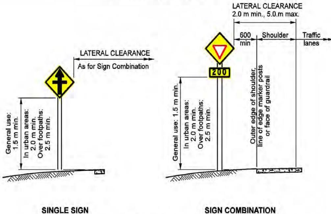
TYPICAL DETAILS FOR ROADSIDE MOUNTED SIGNS (REGULATORY AND WARNING SIGNS) FIGURE 1.3
