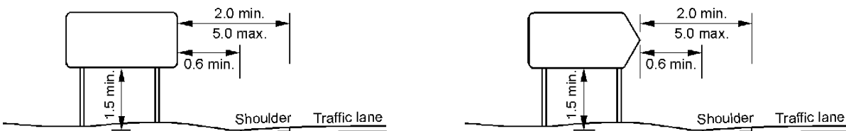
(d) RURAL LOCATION, STANDARD TWO-POLE SUPPORT.
