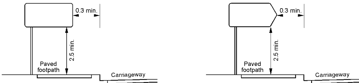
(c) URBAN LOCATION, OVER A FOOTPATH.
